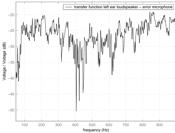
Figure 13: Amplitude of the transfer function between the secondary loudspeaker and the error microphone
