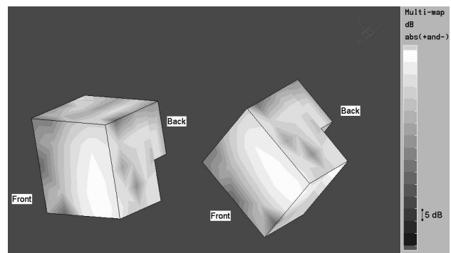
Figure 3: A sound intensity scan inside the cabin (octave band of 125 Hz)
